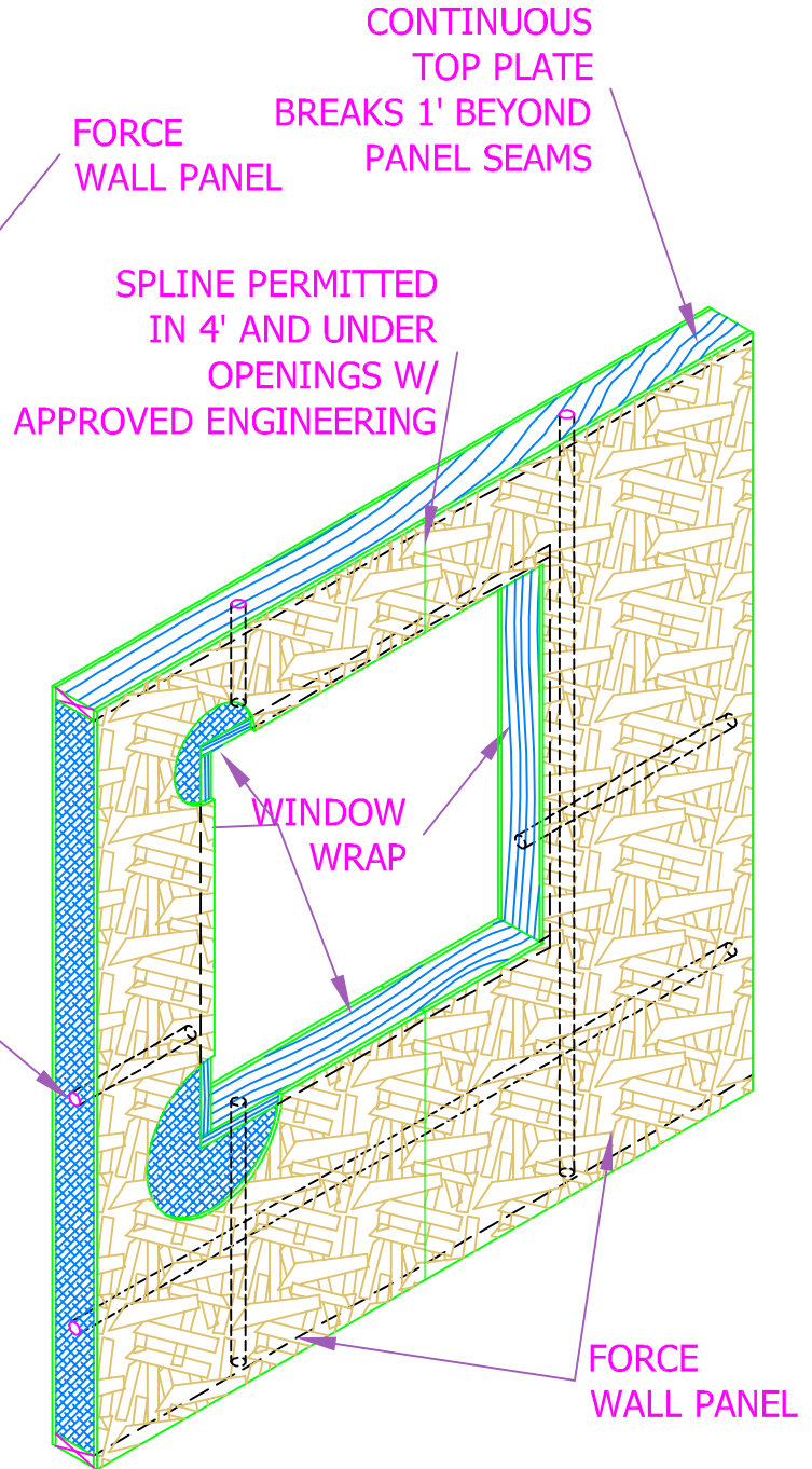
WINDOW WITH PANEL BREAK
