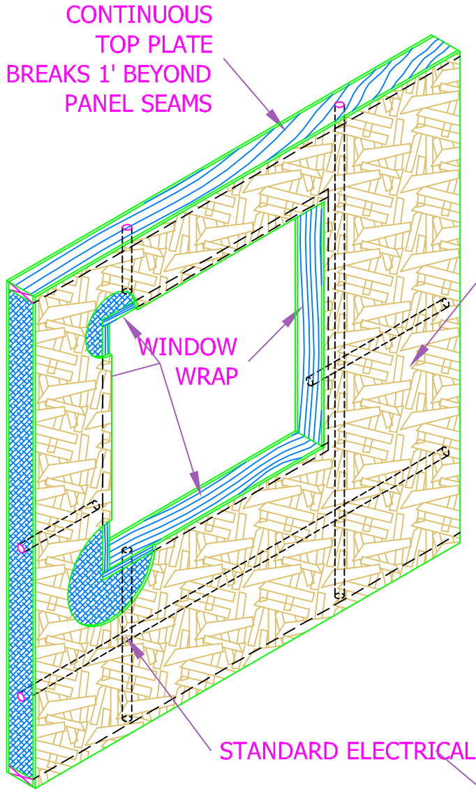
WINDOW WITHOUT PANEL BREAK
